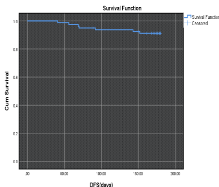
Figure 01: Overall Survival
